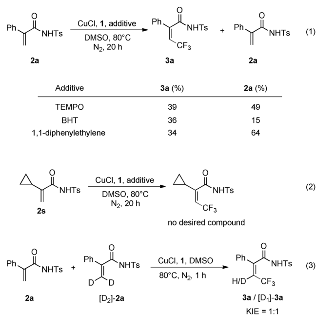
Scheme 4. Control experiments.
